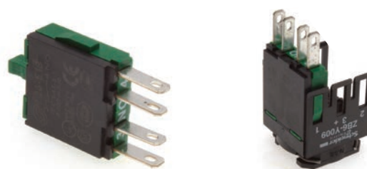
CONTACT BLOCK
