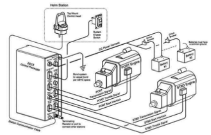
TWIN ENGINES SINGLE STATION
