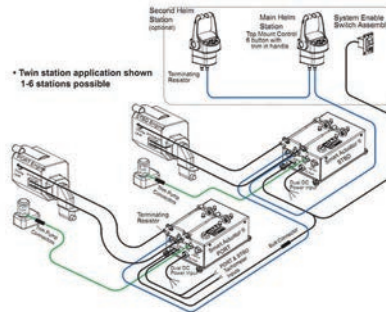
TWIN ENGINES DUAL STATIONS
