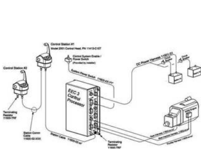
SINGLE ENGINE DUAL STATIONS
